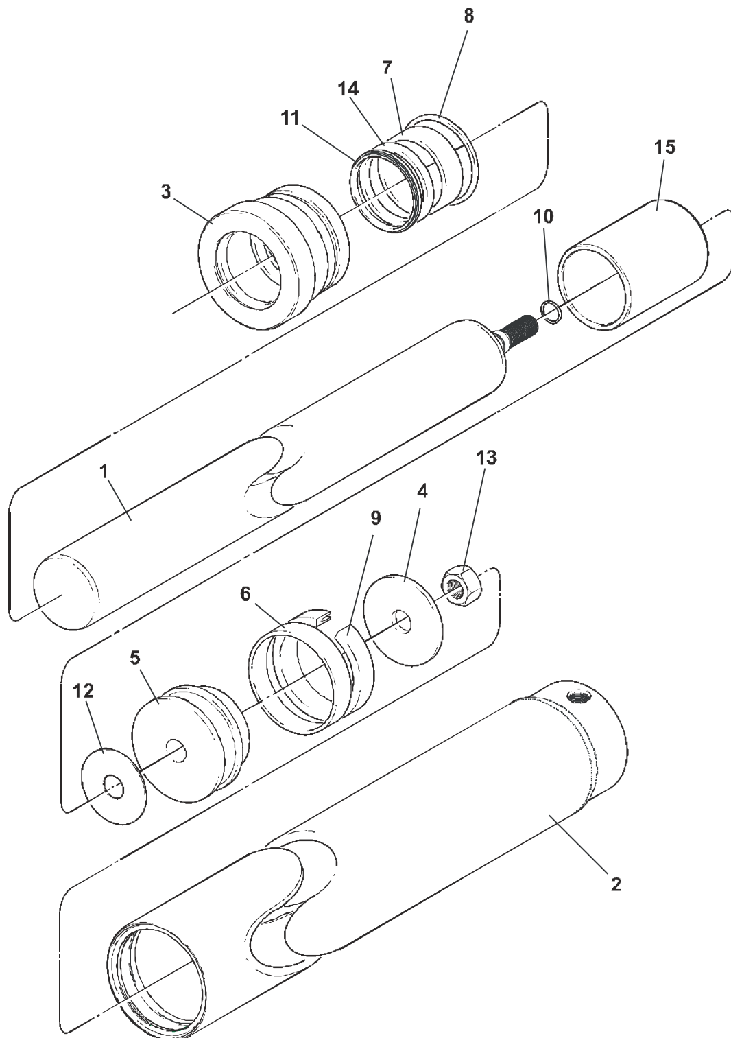
Figure 29 : Lift Cylinder Assembly - 172" Lift Height
