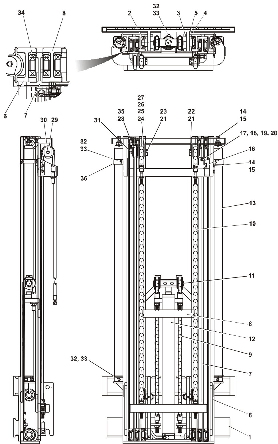
Figure 25 : Full Free Mast and Carriage Assembly - 172" Lift Height
