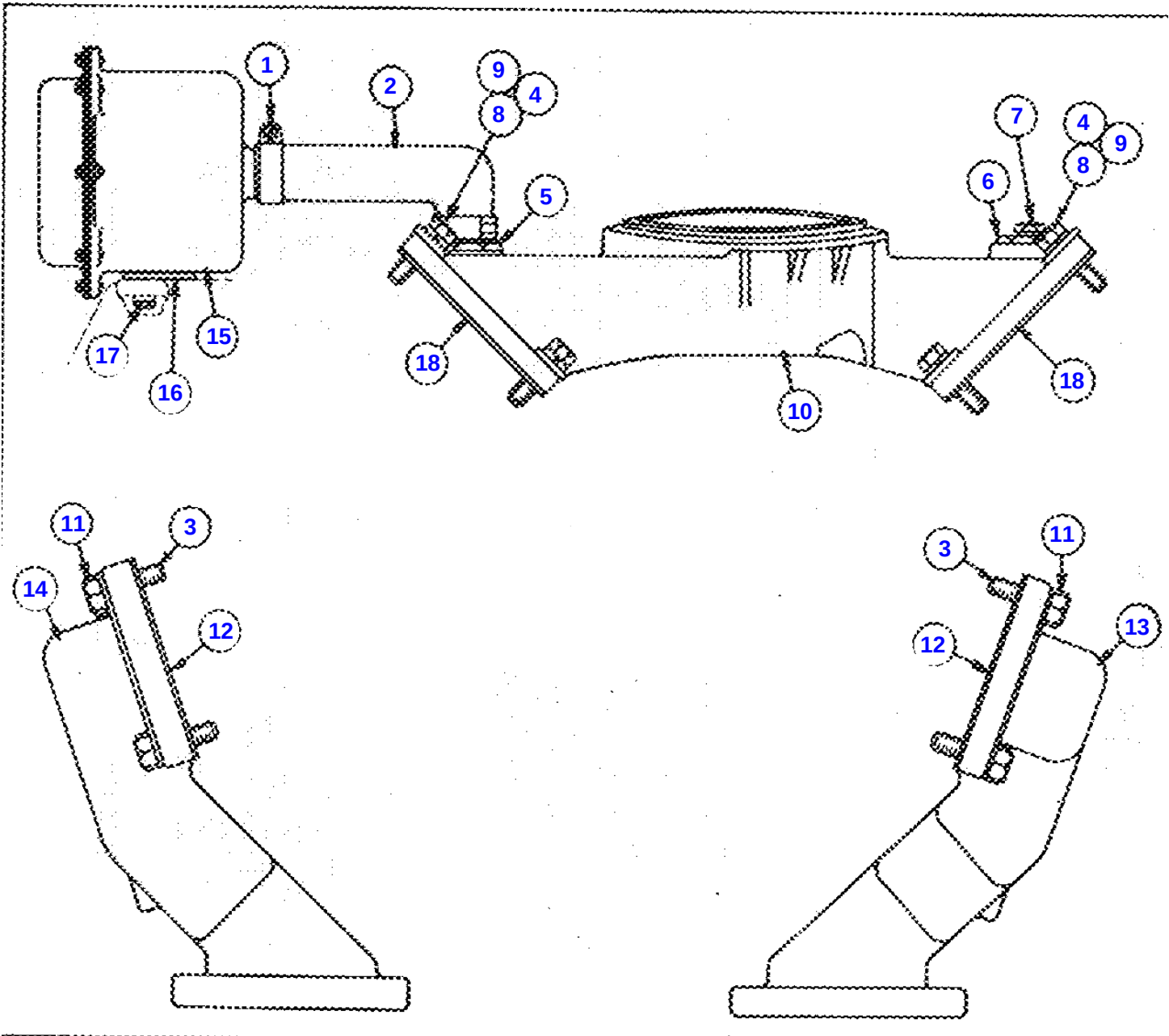
AIR SYSTEM (2N6267 N/S)
